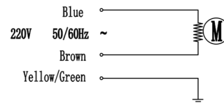
Wiring Diagram
