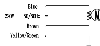
Wiring Diagram
